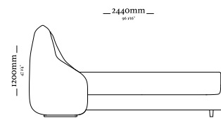
Cama 193 3710 x 2440 x 1200mm
