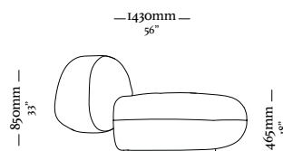
Ass. 2800 2800 x 1430 x 850 c/ almofada
