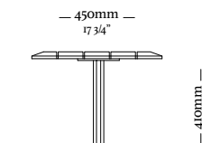
MH 9119 524 x 450 x 410mm
