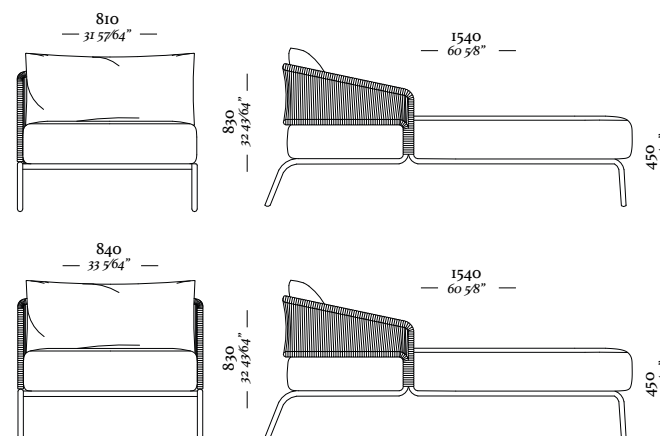
Chaise Longue 1 Braço 810x1540x830mm
