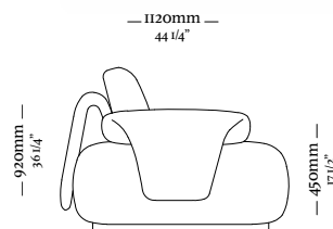
Mod. c/ 1 br ass. 1130 1360 x 1120 x 920mm
